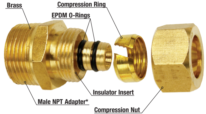
Compression Fitting *1/2" fittings will be indicated by a blue mark
