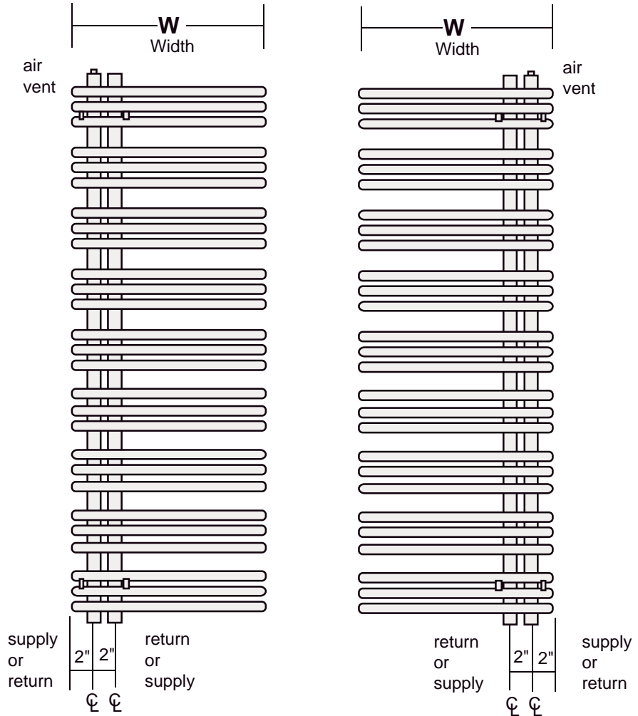
Front View Lefthand & Righthand Dimensions
