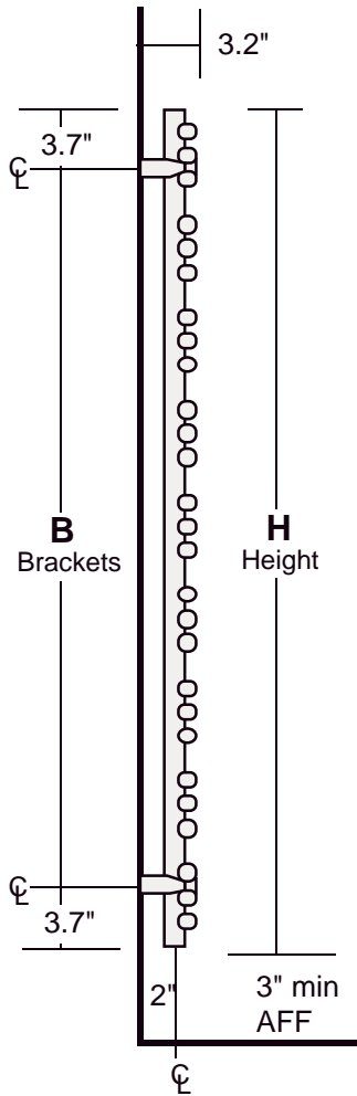
Side View Dimensions
